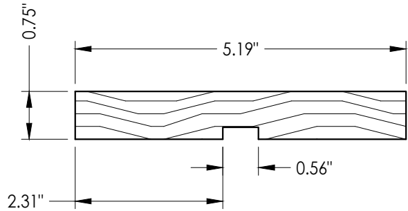
20 FRAME HEADER
