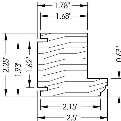
25 SASH STILE
