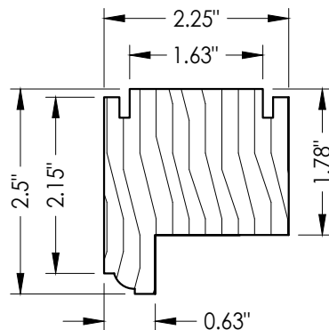
27 TOP SASH TOP RAIL
