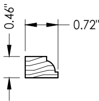
14 GLAZING STOP
